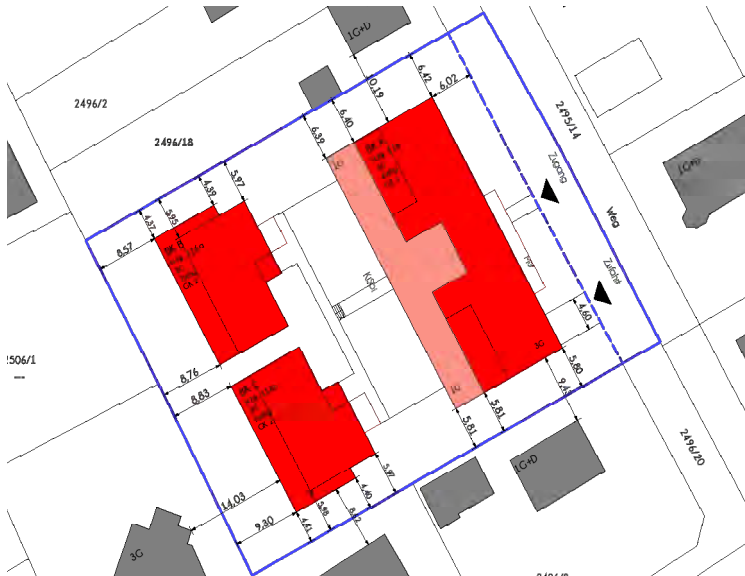
LAGEPLAN | 1_2000
